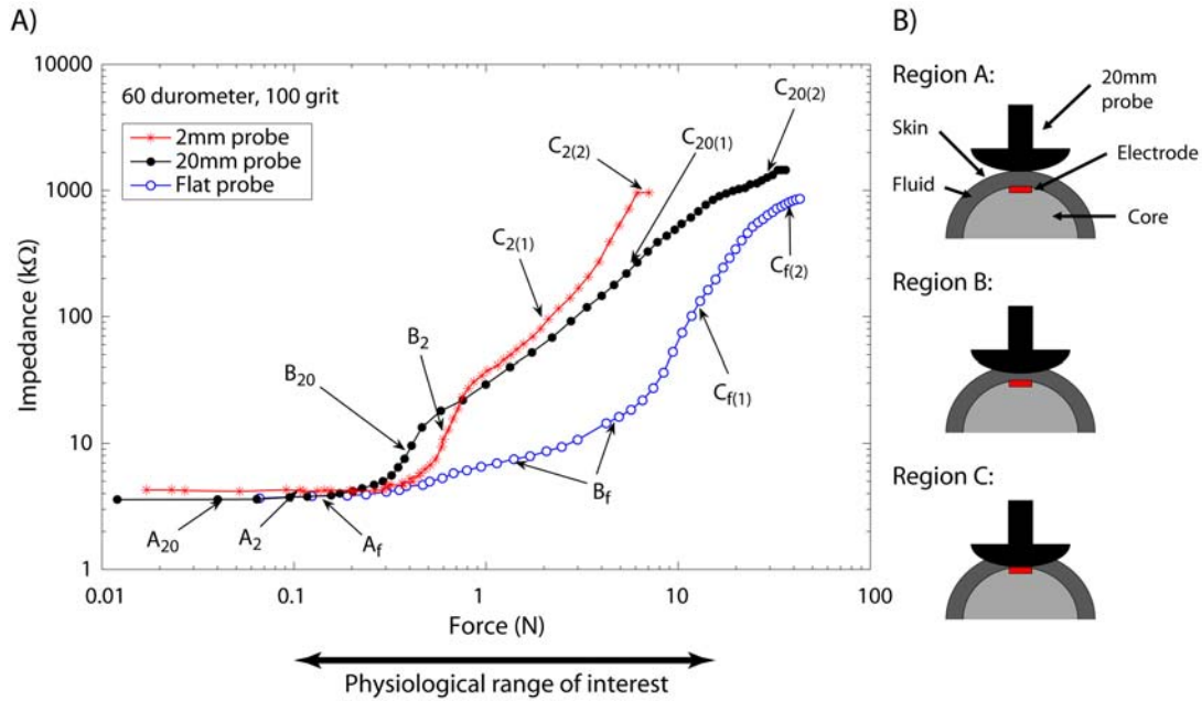
Figure 4: A) Impedance (log scale) as a function of force (log scale) applied normal to the electrode surface. Textured silicone: 60 durometer, 100 grit size. B) Graphic correlating curve shapes to probe indentation (20mm probe shown).
