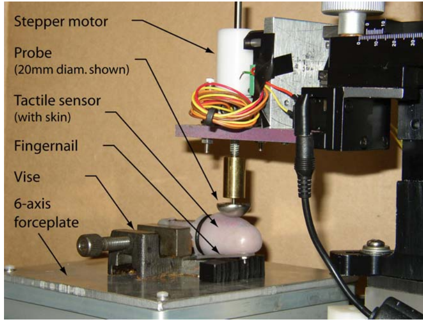
Figure 3: Experimental set-up for static characterization of a single electrode.
