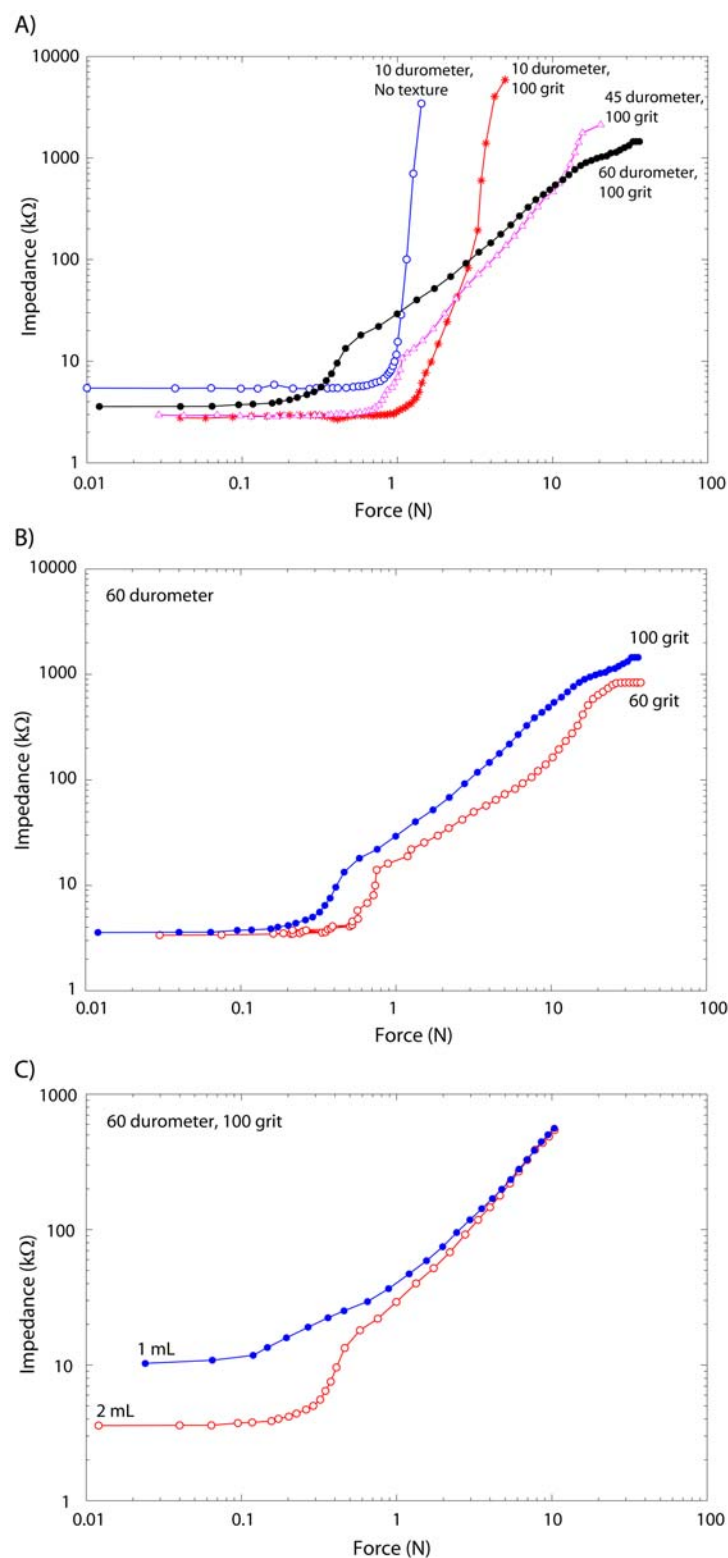
Figure 5: A) Response of sensor to texture stiffness. B) Response to texture depth (grit size). C) Response to fluid volume. Figures A, B, and C show response to the 20mm probe.
