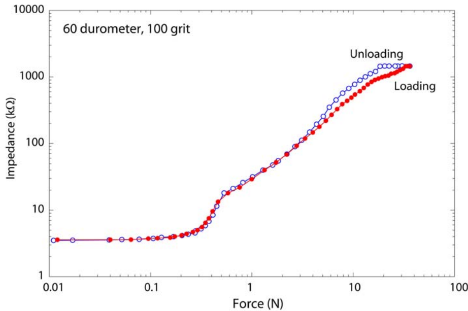
Figure 6: Loading/unloading curve (20mm probe).
