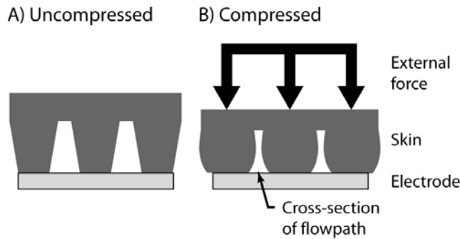
Figure 9: A) The textured rubber is shown in an uncompressed state. B) An applied force compresses the textured rubber and narrows the flowpath of the fluid to the electrode surface. The impedance measured in condition “A” will be lower than that in condition “B.”
