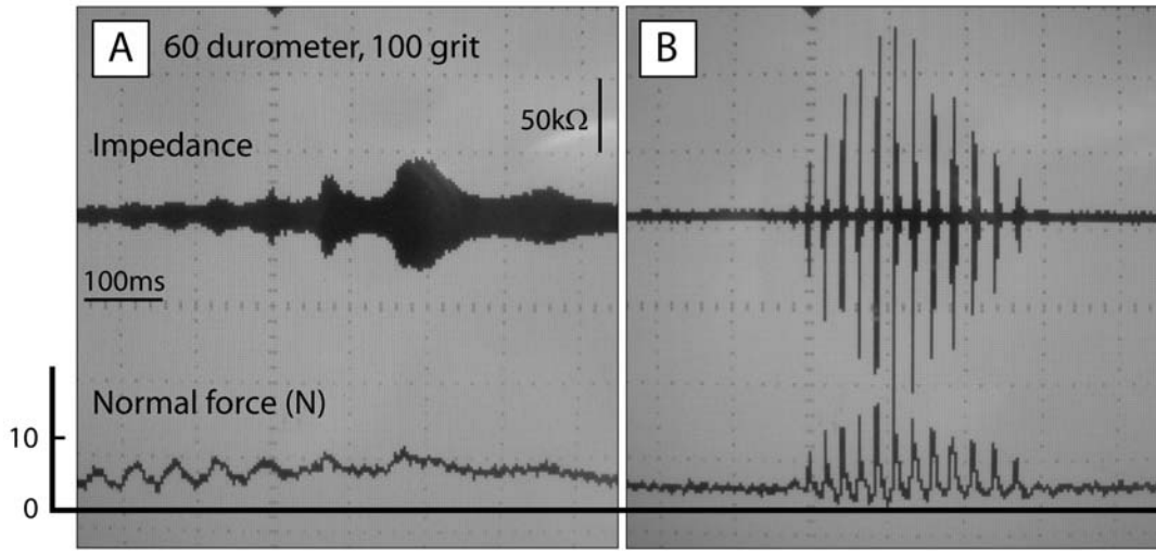
Figure 7: A) 5-15Hz response of sensor. B) 45Hz response of sensor. The force waveform is unidirectional. The impedance waveform is bidirectional because it is capturing the envelope of a sinusoidal waveform.
