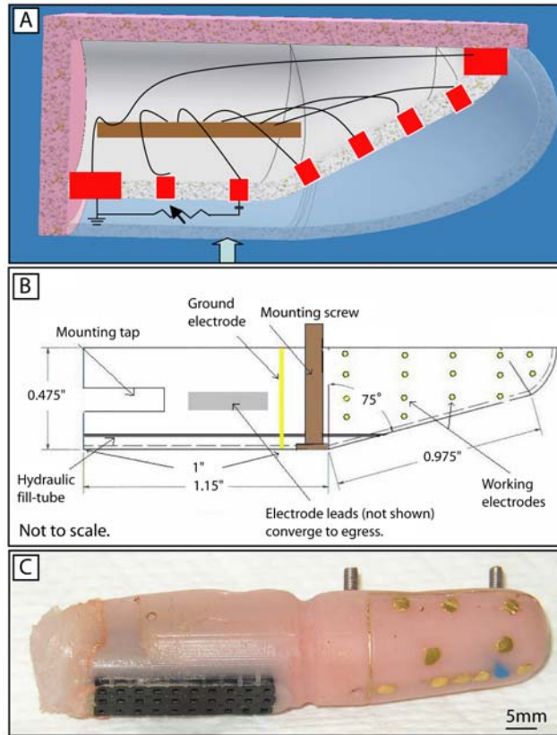
Figure 1: A) Mechanical drawing of the biomimetic tactile sensor showing a rigid core shaped like the distal phalanx (white) with an internal, sealed compartment for electronics (brown) connected to sensing electrodes (red) in contact with a weakly conductive fluid under a viscoelastic skin (light blue). B) Mechanical drawing of the current core design with a sample electrode layout. C) Current acrylic prototype core with skin and fingernail removed. The thin gold ground electrode, circular gold working electrodes, and blue thermistor are visible on the surface of the core.
